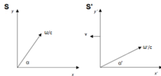
Figure 1- The transformation between the two frames of reference S and S' with the source at the origin. The two frames of reference differ by a velocity v and \alpha is the angle the photon makes with the x-axis. Diagram edited from [3].
