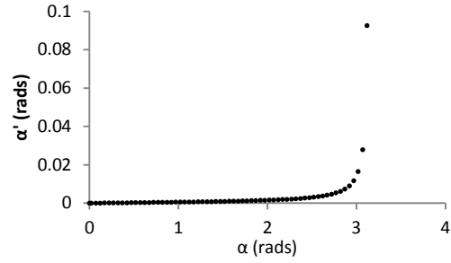
Figure 2- The relation between the emission angle of radiation \alpha from an isotropic point source in frame S and the angle \alpha' as seen by an observer in frame S' .
